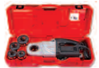
1/2 - 1.1/4" SUPERTRONIC 1250 No. 7.1450
